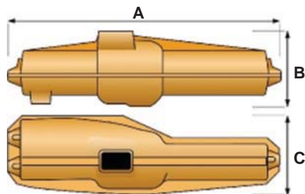
Compression Connector (copper only)
